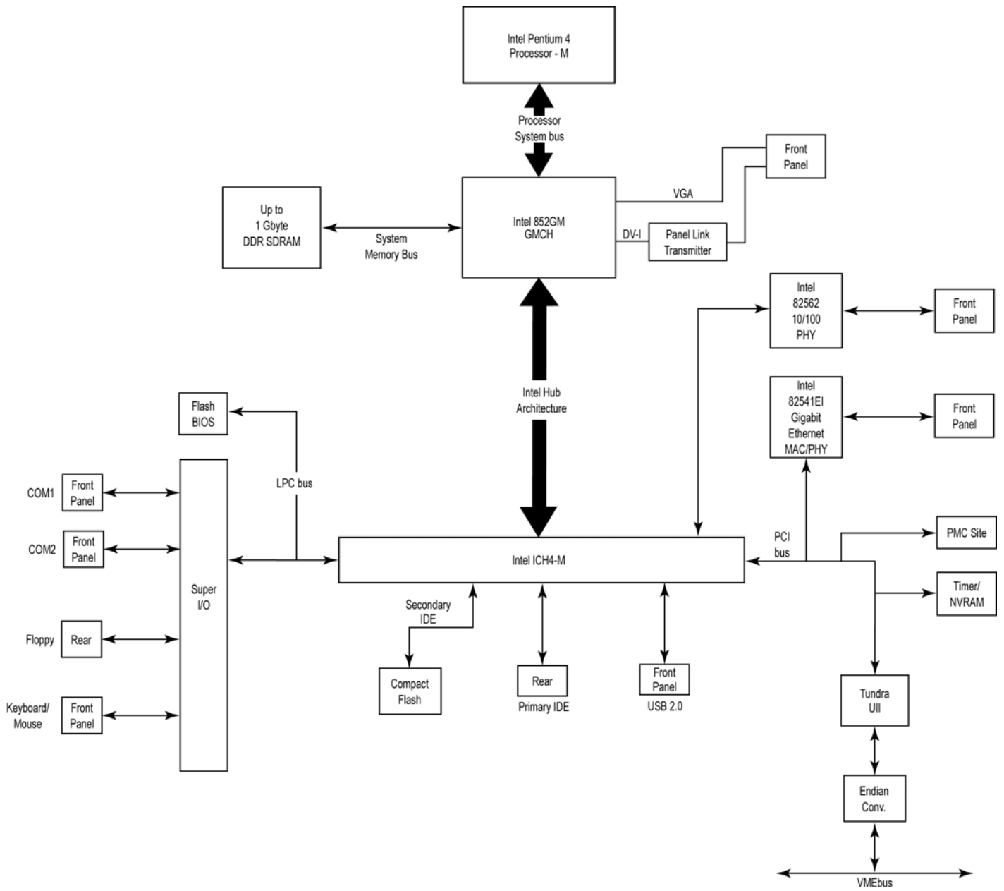
Figure 2. VMIVME-7805 Block Diagram
