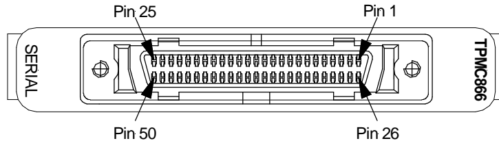
Figure 9-1 : Front Panel I/O Connector Numbering
