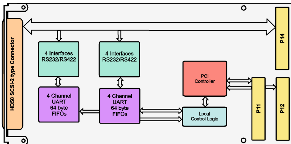
Figure 1-1 : Block Diagram
