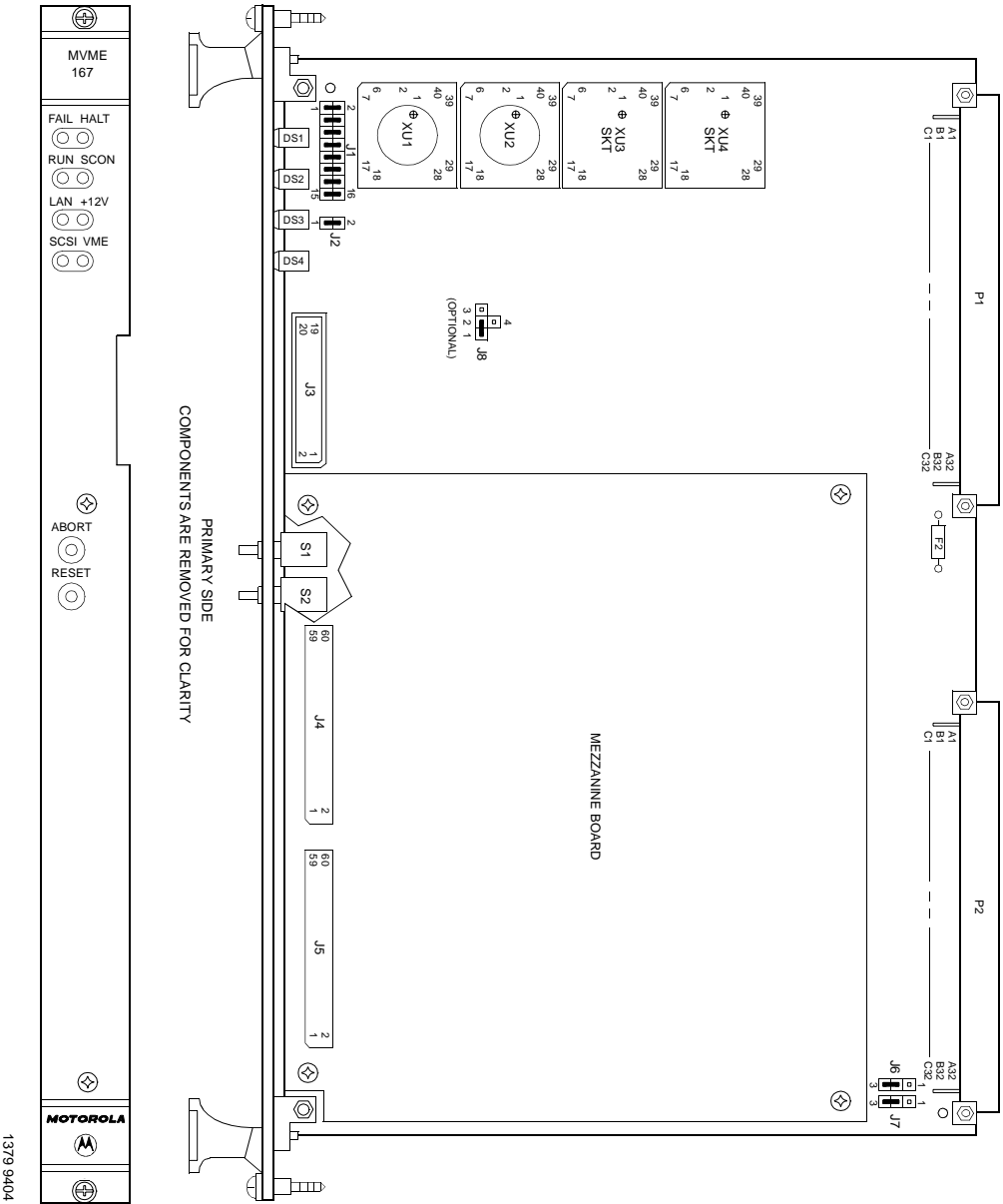
Figure 2-1. MVME167 Switches, Headers, Connectors, Fuses, and LEDs
